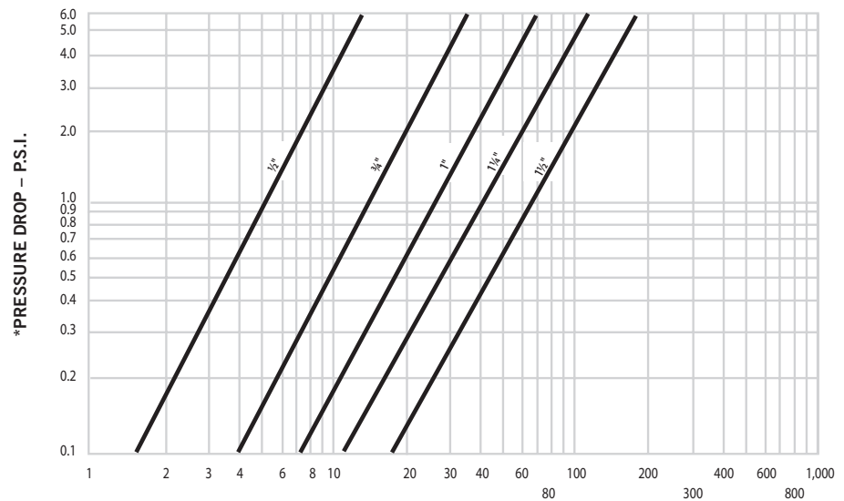
*Frictional losses through branch only. Velocity losses are not included
