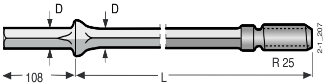
Shank rod, Hex22 - R25
