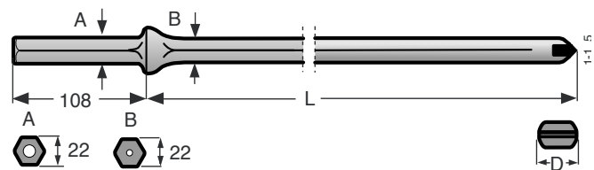
Shank 22x108 mm (7/8" x 4 1/4")
