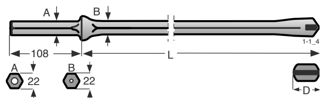
Shank 22x108 mm (7/8" x 4 1/4")
