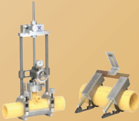
Sidewall Fusion Equipment
