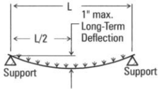
Figure 6-3 Deflection Between Supports
