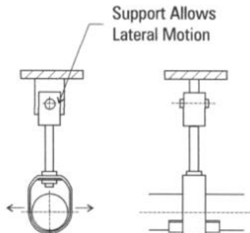
Figure 6-2 Pipeline Hanger
