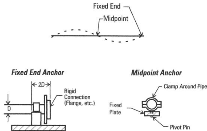
Figure 5-3 Midpoint and End Anchoring
