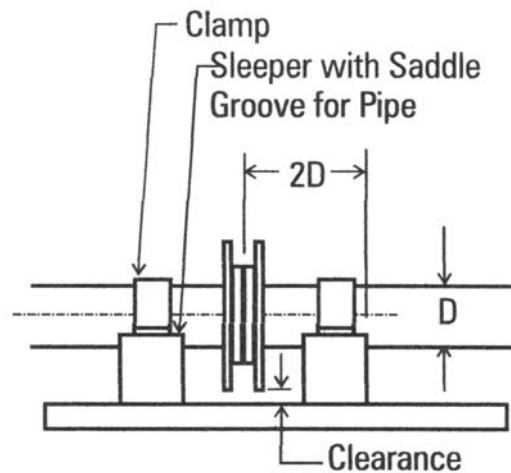
Figure 5-2 Anchoring Flange Connections
